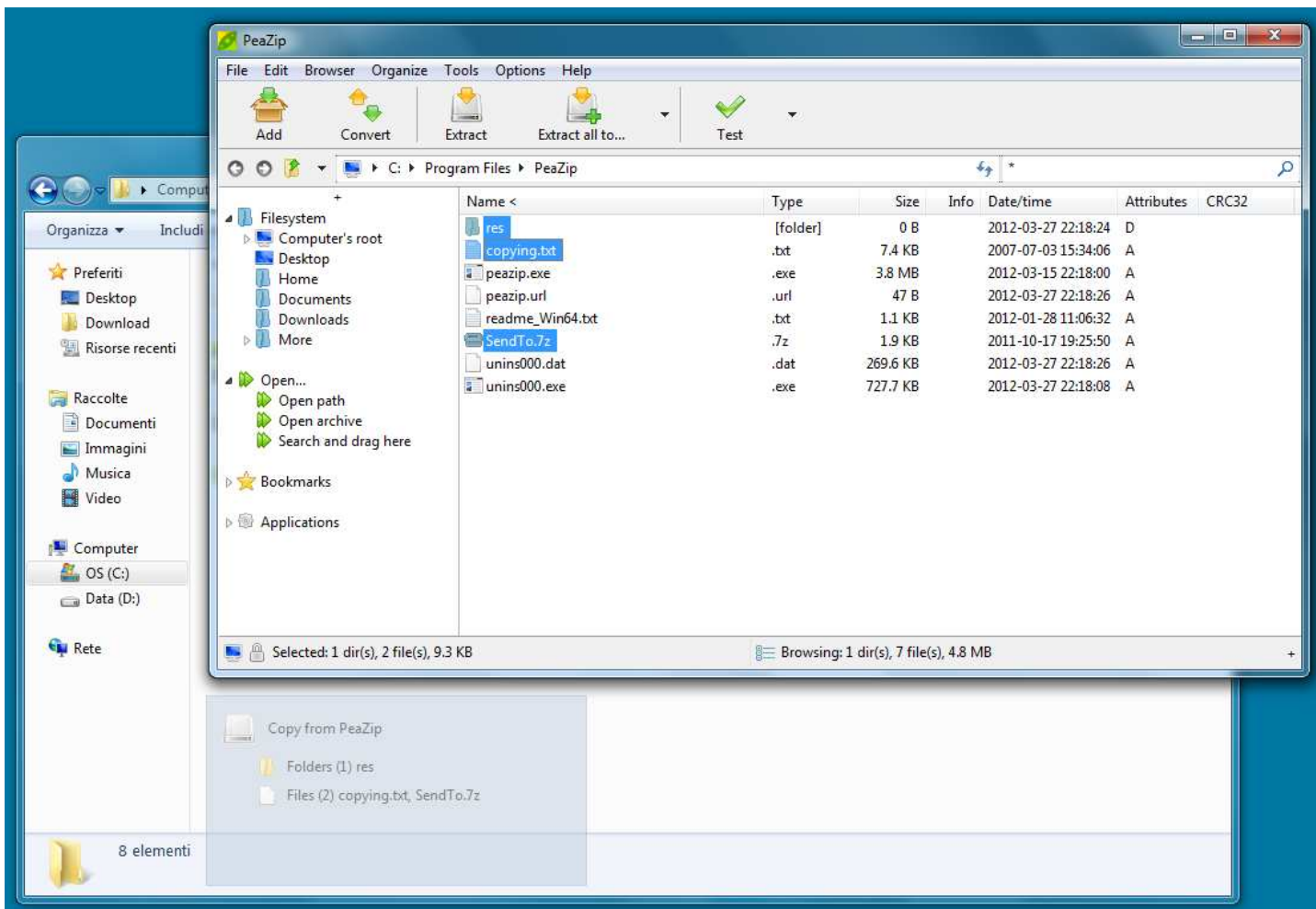
Image 8: drag and drop from application to system (Windows only); files and folders can be dragged from the filesystem or from archives to the desktop or (file)Explorer's windows with Address field enabled (as it is by default on all Windows versions). Drag and drop operations, as well cut/copy selections, are cancelled pressing Esc
