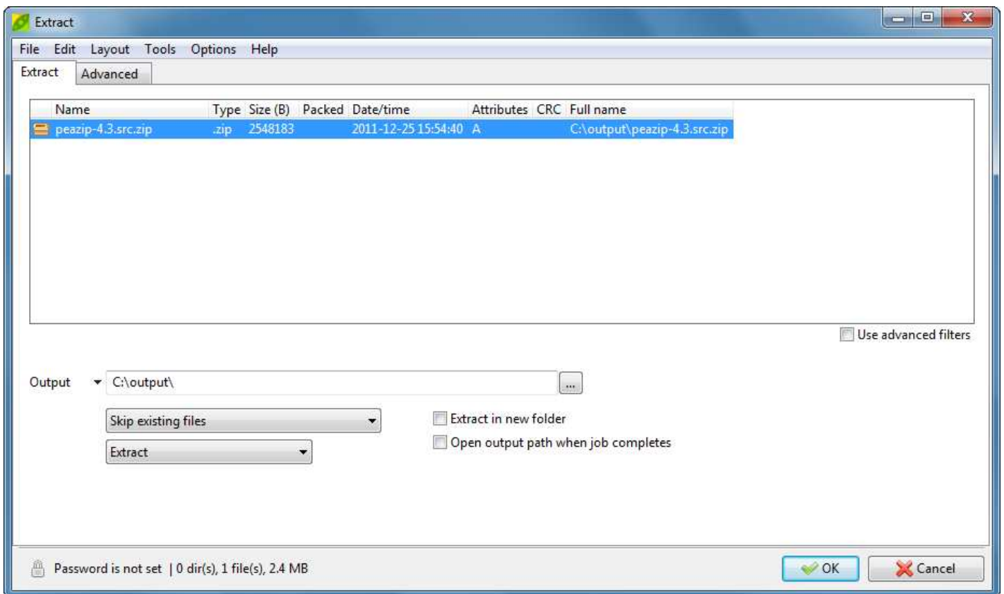
Image 15: Extraction interface, rightclick to display the context menu to add/remove objects from extraction layout, and display other related functions; click on the arrow on the left of the output address for quick selection of the output path in system's paths, favourites, and recently opened directories.
